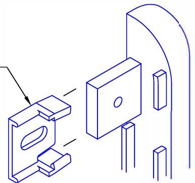
Spacer Detail
