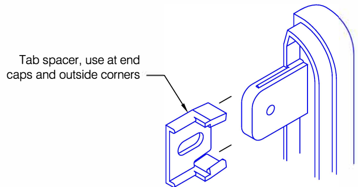
Spacer Detail
