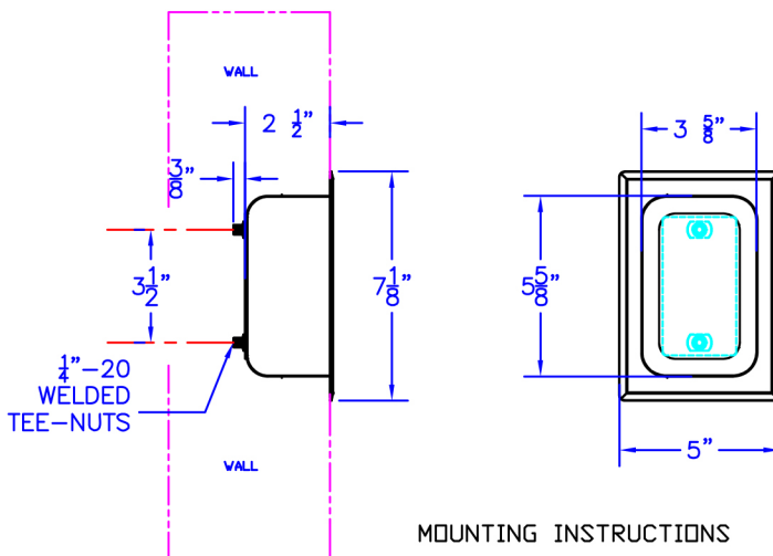
HORIZONTAL MOUNT
